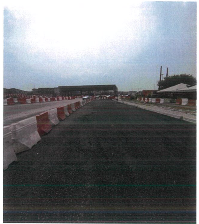
PHOTO 6: Pavement works (Binder course) in progress at CH B
